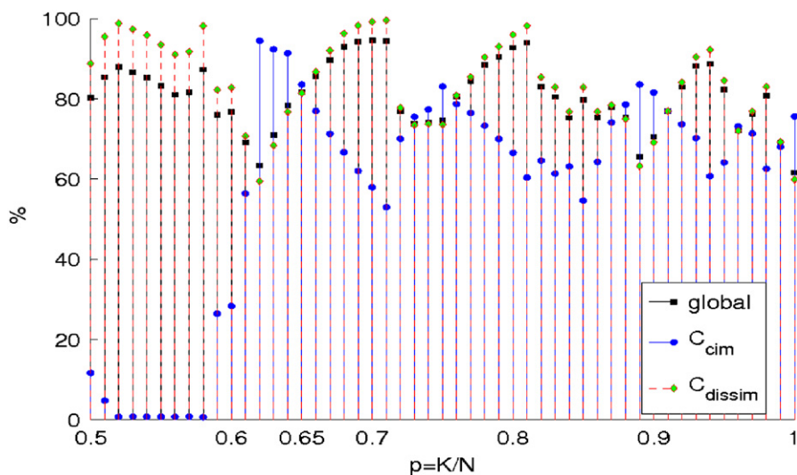
Fig. 9. Graphs of the successful rate for the partial HD (PHD) function of the parameter p = K/N (see formula Section 1.2.1). The graphs stand for the rates for the two classes C_{sim} and C_{dissim} and for all the LDMMaps (global rate).
